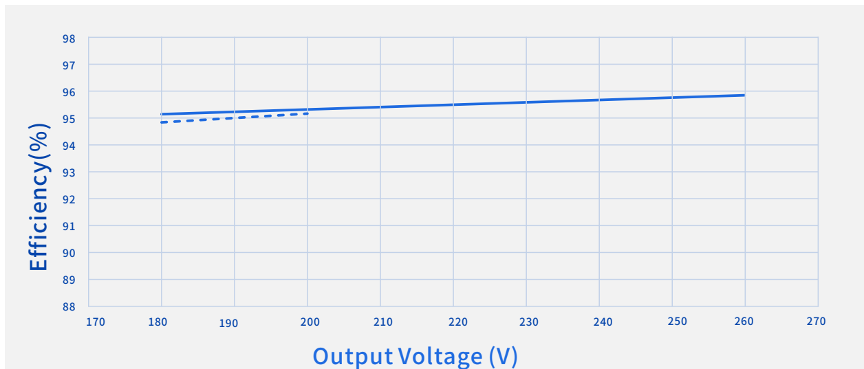
Efficiency Vs. O/P Voltage (Vin=200Vac)
